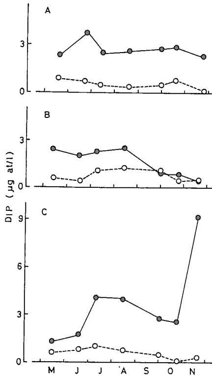
Fig. 12.6 Comparison of the seasonal change of PO 4 -P concentration in inflowing water (black circle) and outflowing water (white circle) in three lagoons (A: Nishinoko Lagoon; B: Komatsunuma Lagoon; C: Katata Lagoon).
