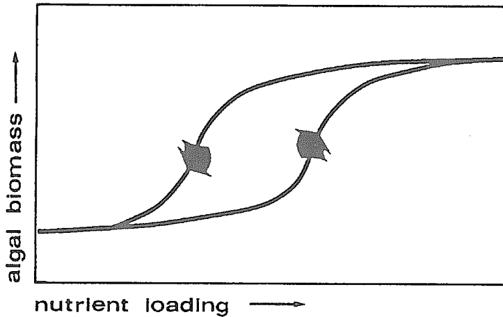
fig. 1.1 Changes in algal biomass with increasing and decreasing nutrient loading: a lake under restoration may have more algal biomass than before restoration. The area within the two curves presents the field of action of biomanipulation (from Hoser, 1989, redrawn).
