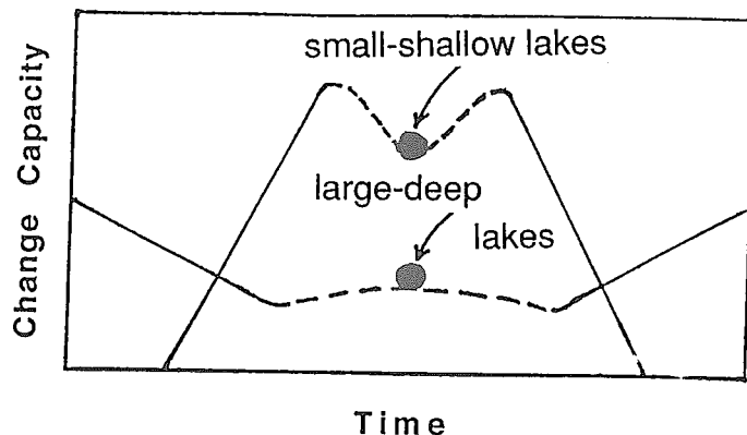
Fig. 3.1 A diagram of lake (small-shallow; large-deep) stability (●) as responded to manipulated (-----) and unmanipulated (—) changes. In large-deep lakes, manipulated alterations are less stable, with lower capacity and longer duration, while unmanipulated changes has longer span and higher stability; in small-shallow lakes its conversely expressed.
