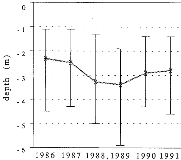
Fig. 8.5 Trend of the annual average of Secchi disc transparency and maximum and minimum values.
