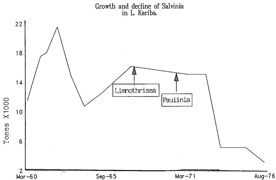
Fig. 13.4 The growth and decline of Salvinia molesta in Lake Kariba, before and after the introduction of Limnothrissa miodon and Paulinia acuminata . Note that the decline of Salvinia was pronounced after the introduction of the grasshopper.
