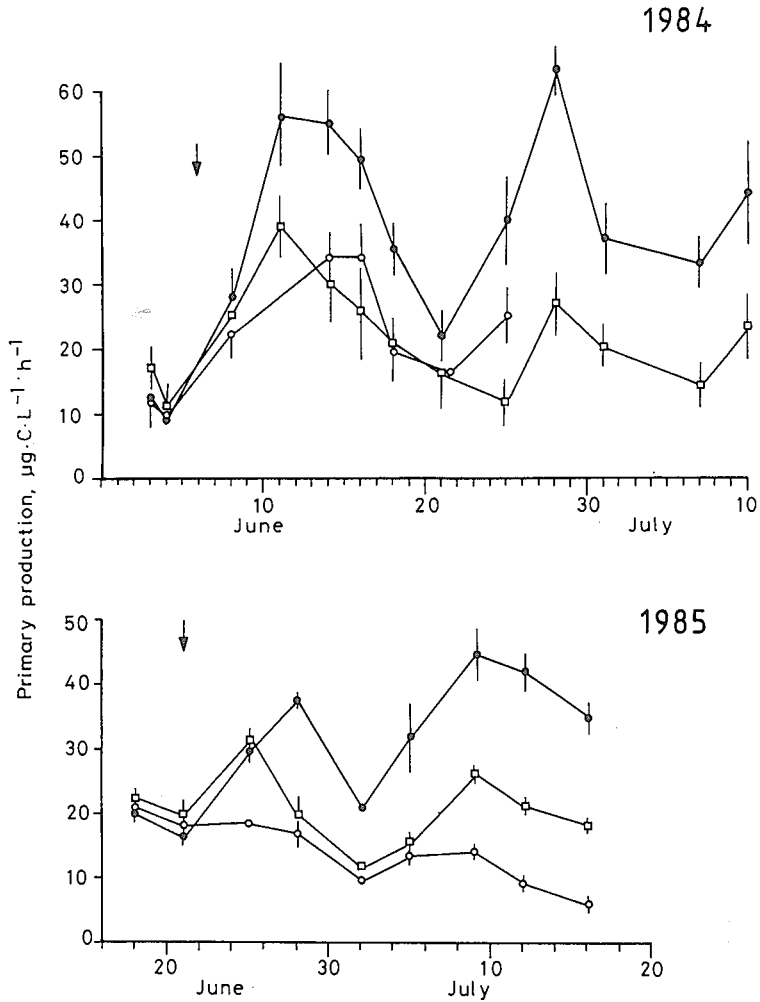
Fig. 10.2 The rates of primary production in the enclosures and in the lake (symbols as in Fig. 10.1).
