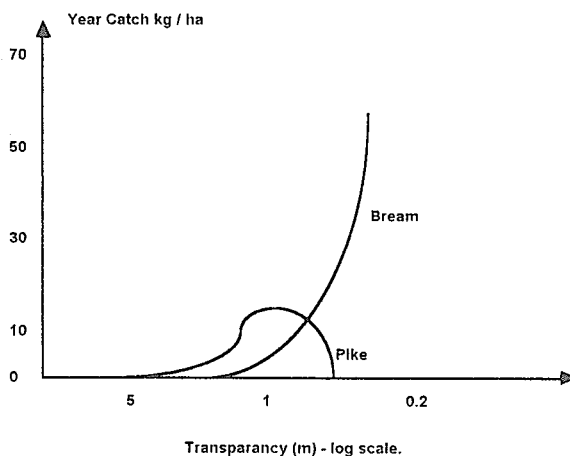
Fig. 7.1 Annual catches of pike and bream ( \text{kg}/\text{ha}^{-1} ) plotted versus transparency (m).
