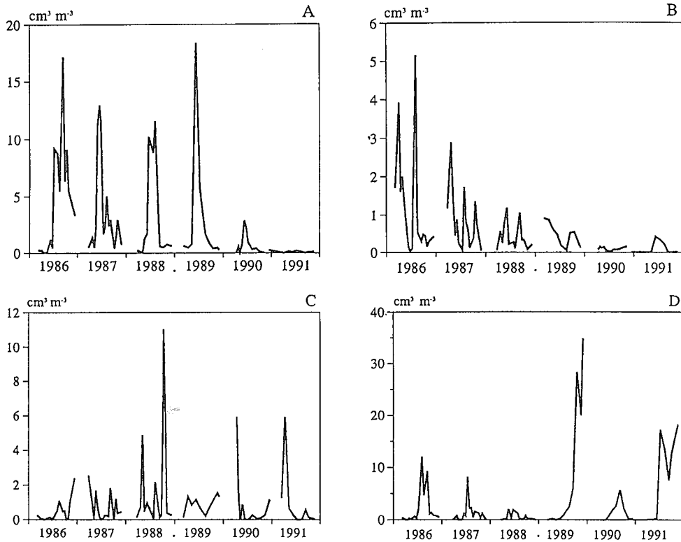
Fig. 8.4 Evolution of the biovolume of the most important algal groups: Chlorophyceae (A), Cryptophyceae (B), Chrysophyceae (C), Cyanophyta (D).
