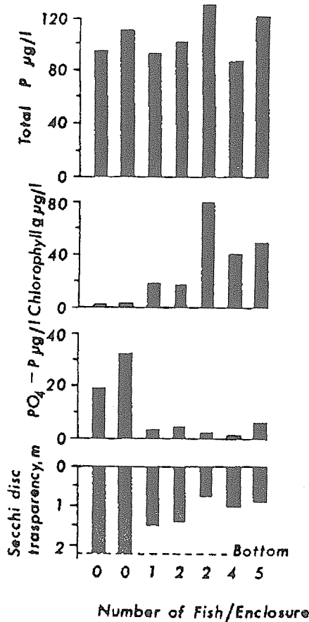
Fig. 1.4 The effect of increasing fish stock on water transparency, chlorophyll-a and phosphate concentrations in plastic bags containing similar concentrations of total P. The evidence for eutrophy is most marked when more fish are present (from Lynch, 1975, redrawn).
