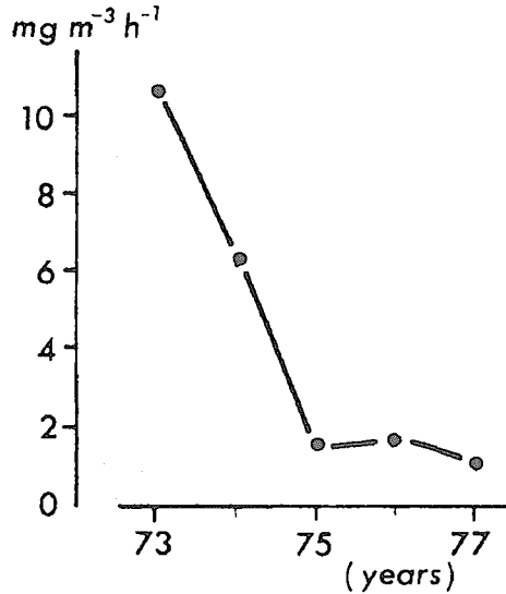
Fig. 1.5 Lake Lilla Stockelidsvatten; limnetic primary production. Mean mid-day values. The removal of fish by rotenone in November 1973, determine a decrease in primary production, (from Henrikson et al. , 1980, redrawn).
