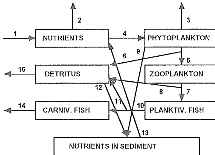
Fig. 7.7 The model used as an experimental tool in this Section is shown. The state variables are nutrients (only phosphorus is considered in this case), phytoplankton, zooplankton, plantivorous fish, carnivorous fish, nutrients in sediment and detritus. The processes are: 1. inflow of nutrients, 2. outflow of nutrients, 3. outflow of phytoplankton, 4. uptake of nutrients by phytoplankton for growth, 5. grazing, 6. loss of detritus by grazing, 7. predation on zooplankton, 8. loss of detritus by this predation, 9. settling of phytoplankton, 10. predation by carnivorous fish, 11. loss of detritus by this predation, 13. release of nutrients from the sediment, 14. catch of fish, 15. outflow of detritus.
