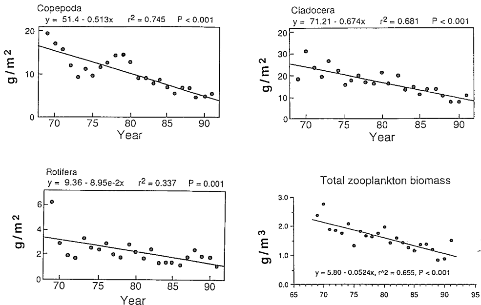
Fig. 11.3 Annual (1969-91) averages of Copepoda, Cladocera and Rotifera biomass ( \text{g}_{(ww)} \text{m}^{-2} ) and total zoomass ( \text{g}_{(ww)} \text{m}^{-3} ). Regressions between parameters and time are given.
